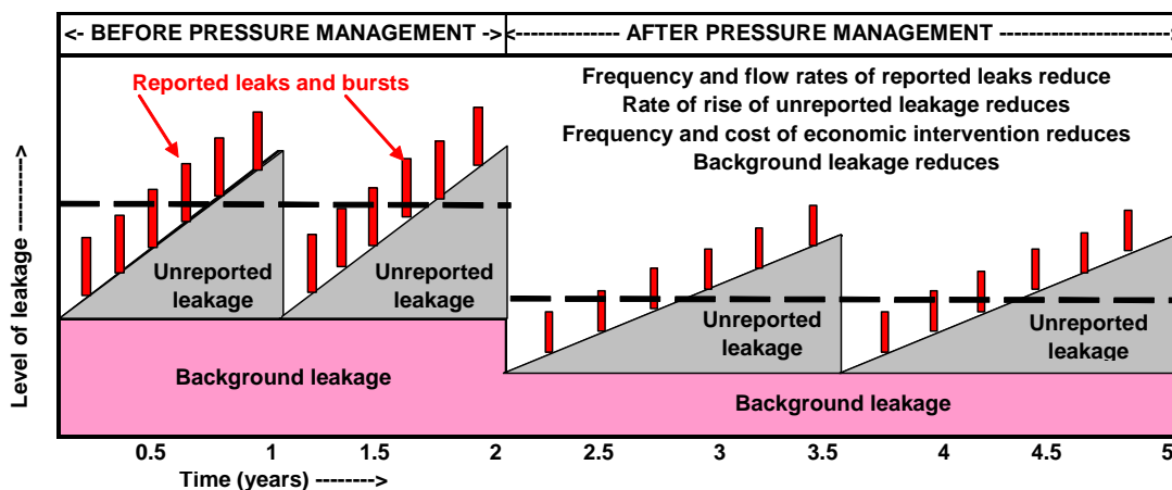
Figure 1: Influence of pressure management on BABE components of Real Losses
