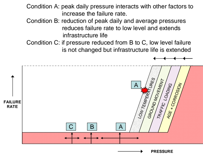
Figure 3: Influence of pressure management on break frequency of mains and services
